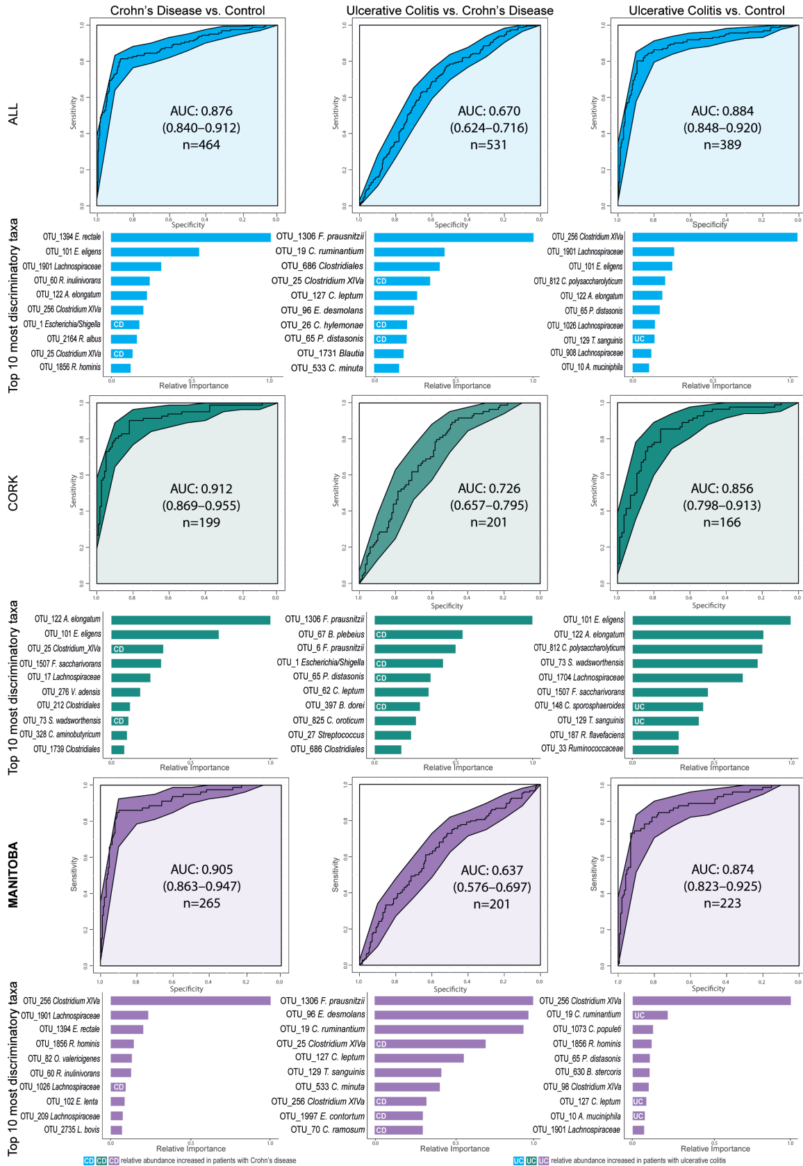
Figure 3 Machine learning classification of the subject cohorts, first combined and then separated by geographic location. Receiver operating characteristic curves (ROC) for the boosted tree models on the bases of proportional normalised operational taxonomic units (OTUs) present in >5% of samples. Below each ROC curve, variable importance plots show the relative importance for the 10 OTUs with the highest gain for each comparison alongside their highest known classification. The white UC and CD labels within the bars indicate which OTUs are increased in their respective patient group, bars without mark indicate that their respective taxon is increased in the other class of the model. A model with an area under the curve (AUC) of 0.5 has no discriminatory capacity, whereas an AUC of 1 indicates perfect separation of the response variables.
