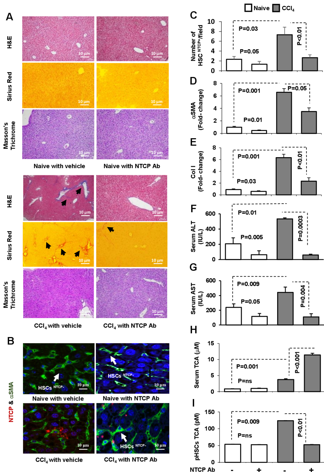
Figure 5 NTCP neutralizing antibody inhibited LF in mice model of CCl 4 . LF was induced in C57/BL mice for 8 weeks and was compared with naive counterparts ( n=10 in each group; experiment repeated three times). NTCP neutralizing antibody was intraperitoneally injected at week 6 of CCl 4 for an additional 2 weeks as described in Materials and methods section. Representative sections of immunohistochemical liver staining with (A) H&E, Masson's trichrome and Sirius red (original magnification 10 \times ). (B) Immunofluorescent visualisation of HSCs on liver sections obtained from untreated and treated mice. HSCs are shown as follows: DAPI conjugated the nucleus (blue), Cy-2 conjugated \alpha SMA (green), Cy-3 conjugated NTCP (red) that quantified in (C). Liver injury markers of (D) \alpha SMA mRNA, (E) collagen mRNA, (F) serum ALT, (G) serum AST, (H) serum TCA and (I) pHSC TCA were assessed. ALT, alanine transaminase; \alpha SMA, alpha smooth muscle actin; AST, aspartate transaminase; LF, liver fibrosis; NTCP, sodium taurocholate cotransporting polypeptide; pHSCs, primary hepatic stellate cells; TCA, taurocholic acid.
