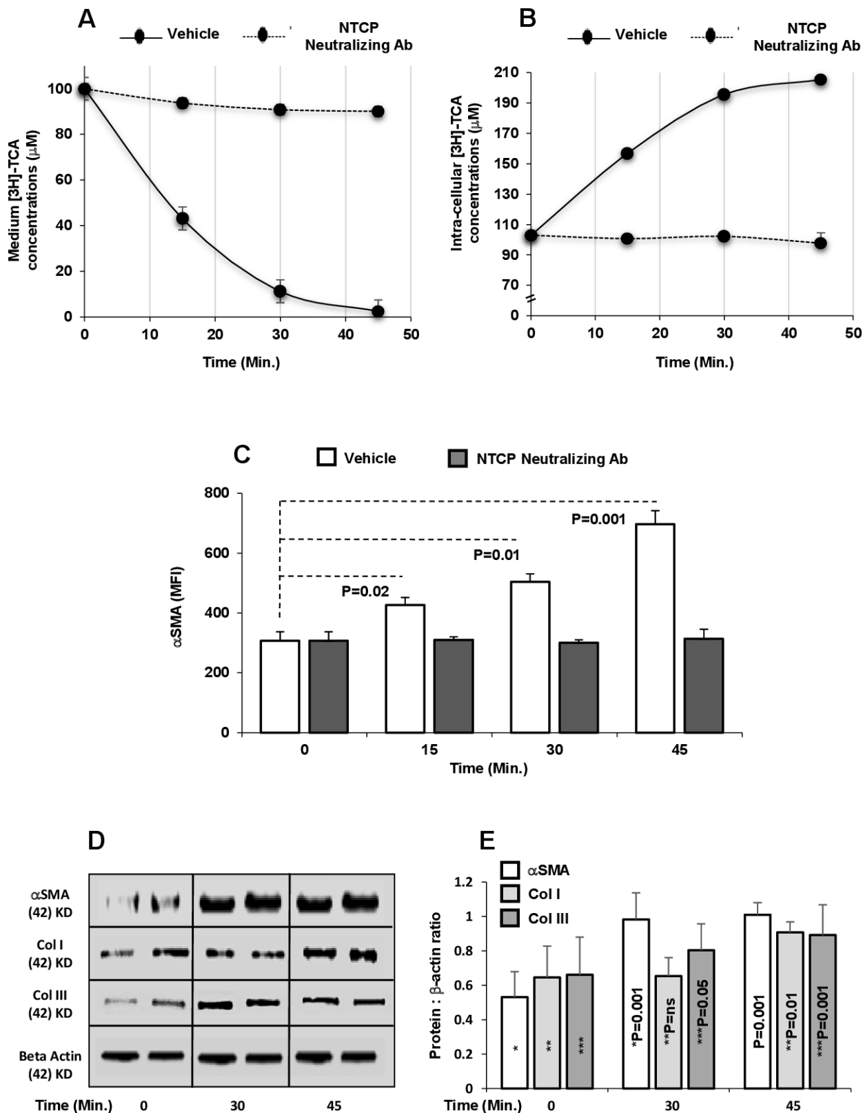
Figure 2 TCA trafficking in HSCs. Sorted LX2 NTCP+ cells were incubated with buffer containing 100 μM TCA supplemented with radiolabeled 0.25 μCi [3H] TCA with or without NTCP blocker (neutralizing antibody) for 15, 30 or 45 min. Kinetics of TCA concentrations in (A) medium and (B) cell lysate made by scintillation counting. Kinetics of MFI of LX2 NTCP+ αSMA of 15 min time intervals following TCA insults with or without NTCP neutralizing antibody performed by (C) flow cytometry, (D) western blots of fibrosis markers (αSMA, Col I and Col III (following 30 and 45 min)) and (E) quantitated through protein:β-actin ratio. Results between groups were statistically significant (p<0.05). αSMA, alpha smooth muscle actin; MFI, mean fluorescence intensity; NTCP, sodium + /taurocholate cotransporting polypeptide; TCA, taurocholic acid.
